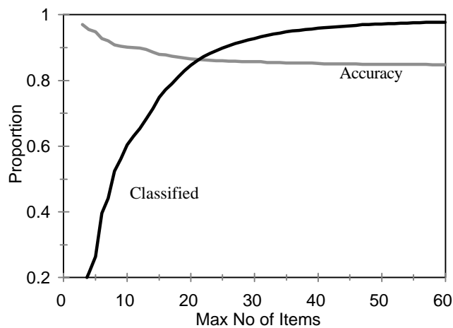
Figure 3: Proportion of examinees classified and the accuracy of those classifications as a function of the maximum number of administered items (state-NAEP items, four latent states, sequential testing using information gain, sequential decisions using SPRT).
